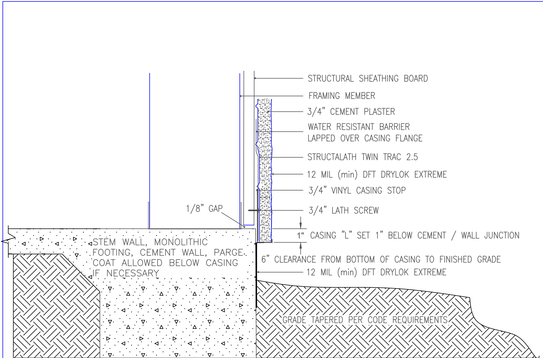
SCS 02_02 FRAME TO FOUNDATION TERMINATION USING CASING
