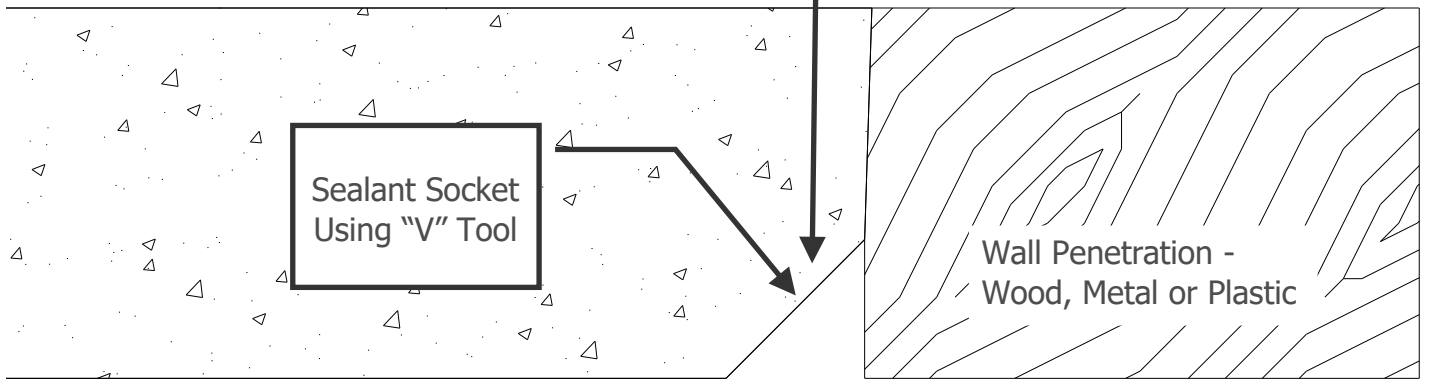
Figure 7-1 Sealant Socket 3/8" width X 3/8" Deep
