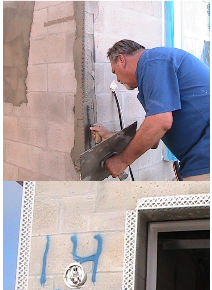
Figure 8-4 - Author demonstrating how to properly "prep" a corner bead to eliminate backside voids. Bead applied to a concrete block wall.
