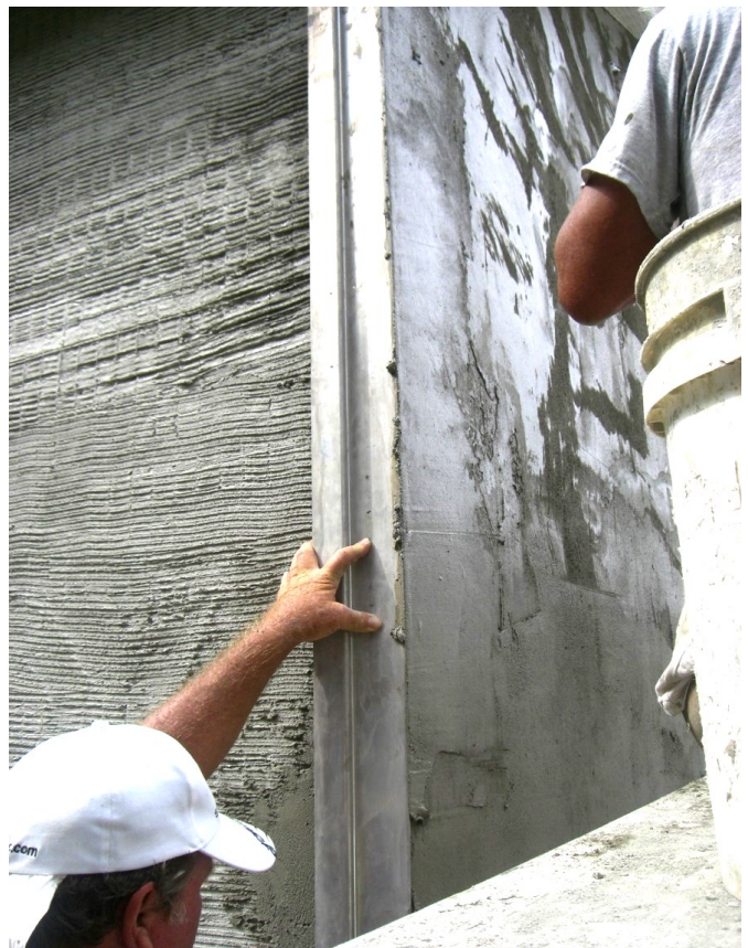
Figure 8-9 Using a Feather Edge Rod to form an External Corner. "Rodding a Corner".
