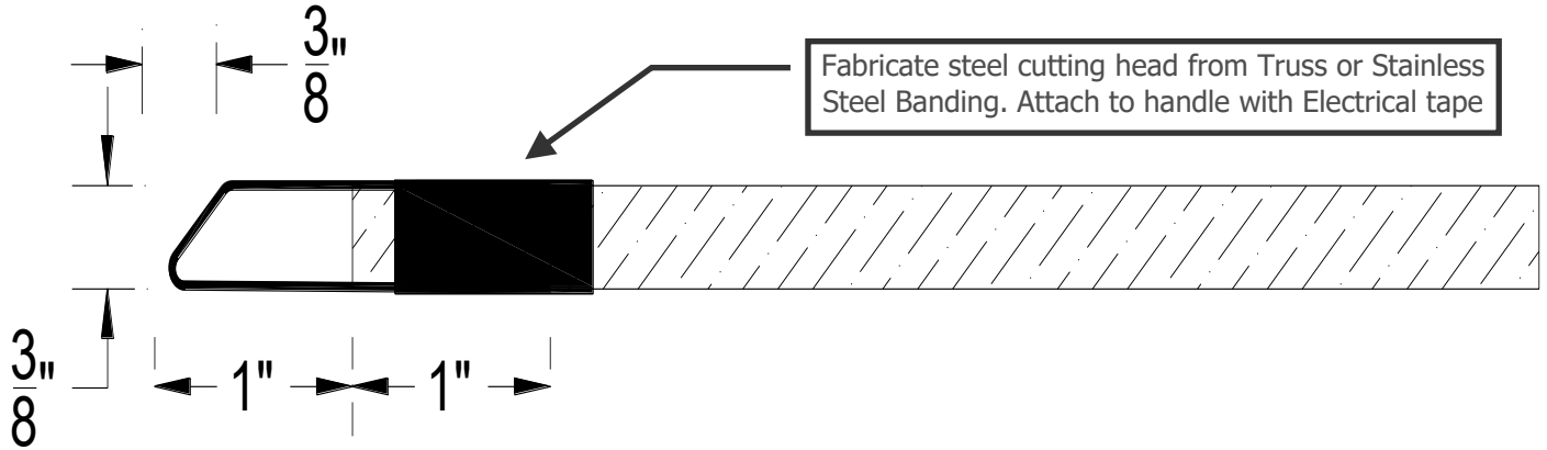
Figure 7-5 Cutting the Sealant Socket with the "V" tool. Two (2) - 3/16" deep passes are made to ensure a smooth socket
