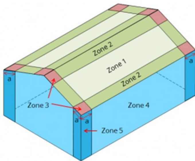
Figure 4-1 Pressure Zones for Walls
